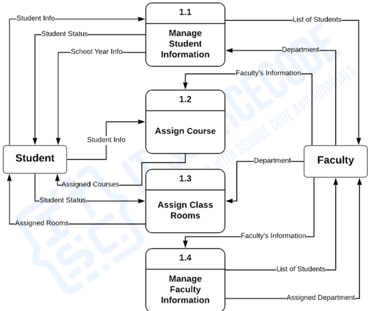
University Management System DFD Level 1
