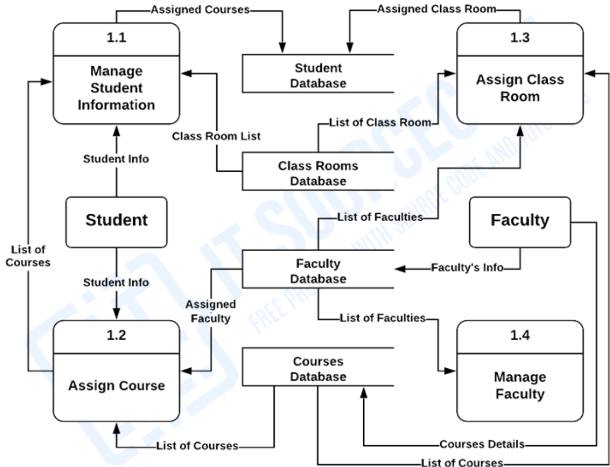
University Management System DFD Level 2
