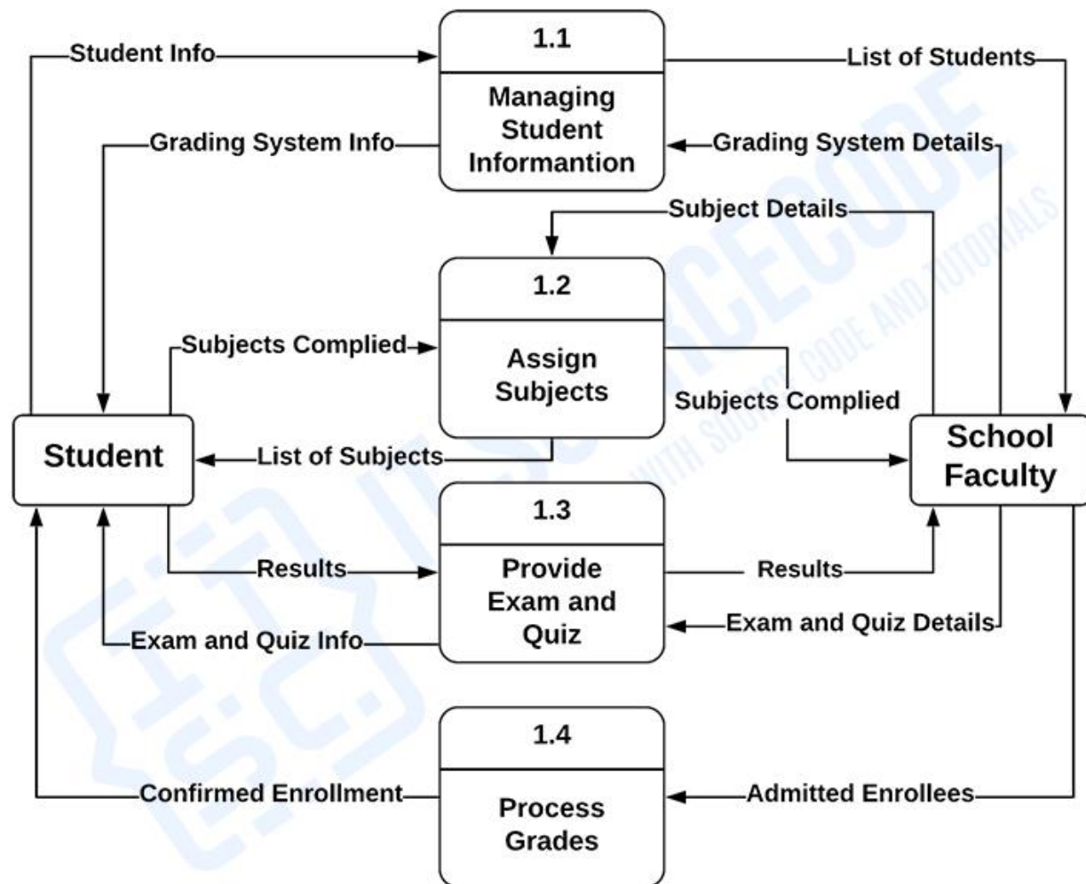
Level 1 DFD for Student Grading System
