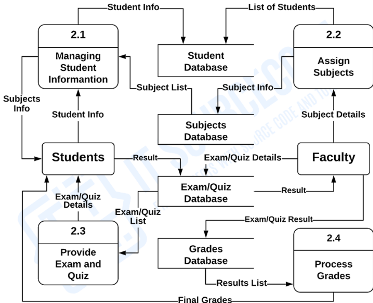
Level 2 DFD for Student Grading System
