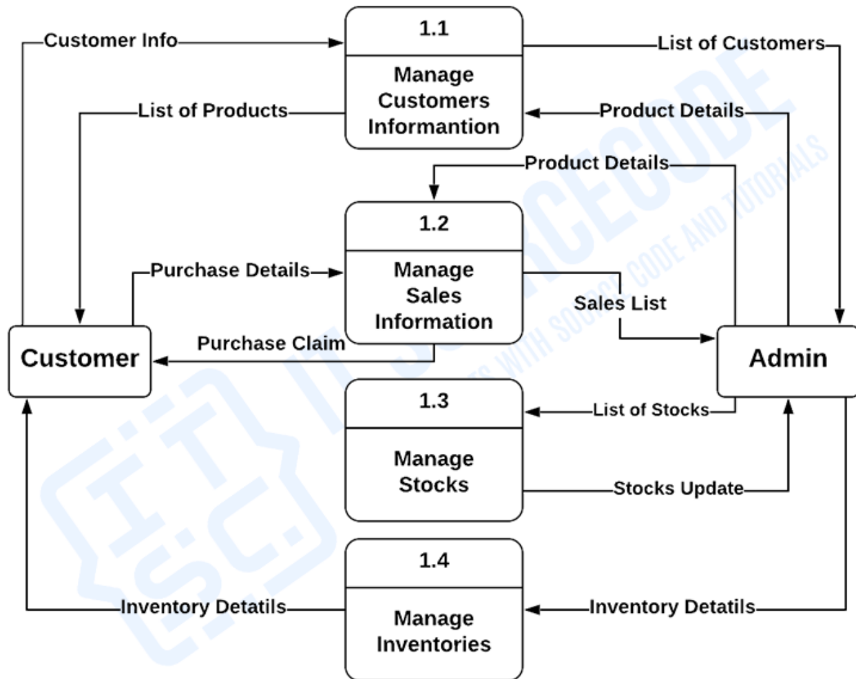
Level 1 DFD for Sales and Inventory System
