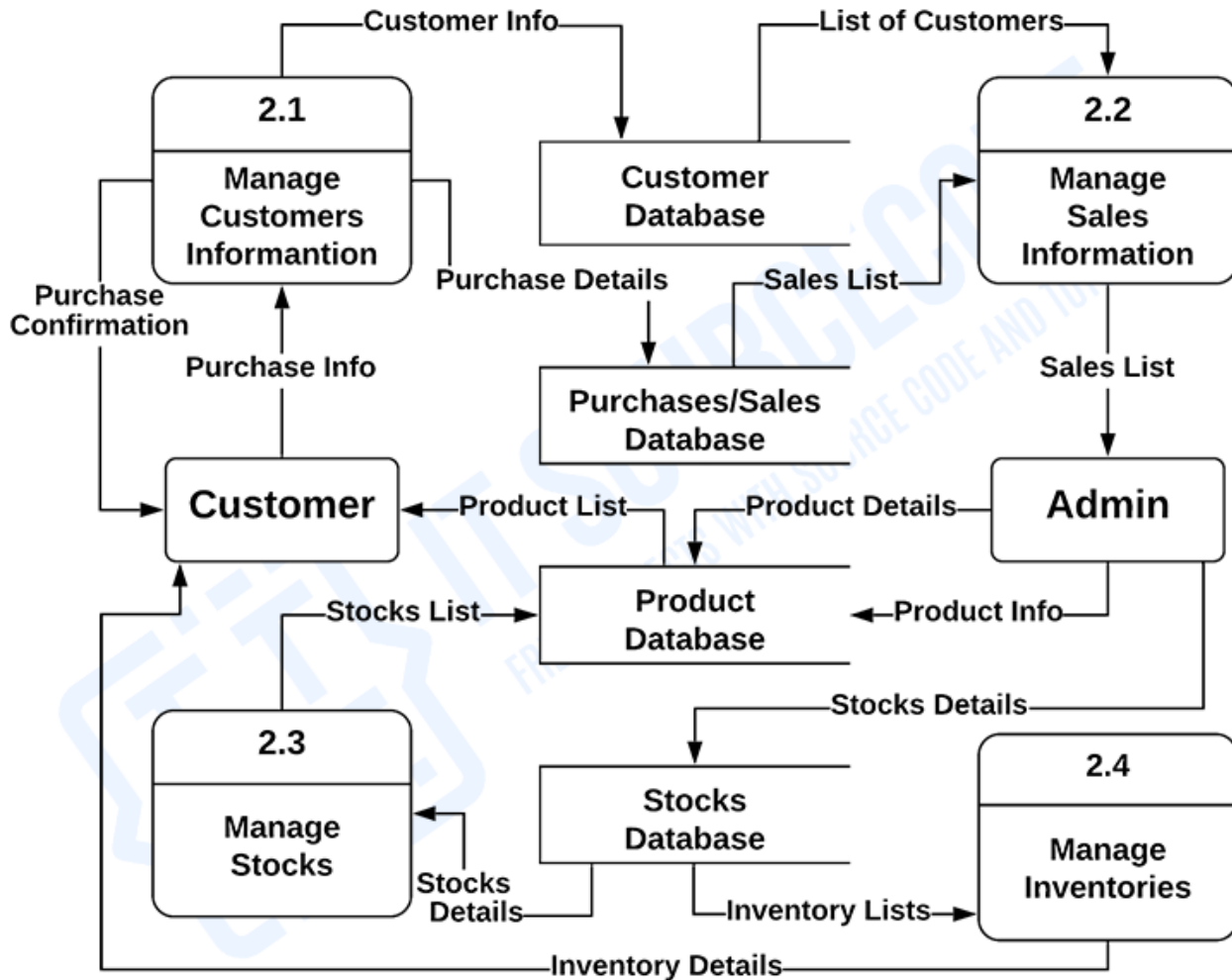
DFD Level 2 for Sales and Inventory System
