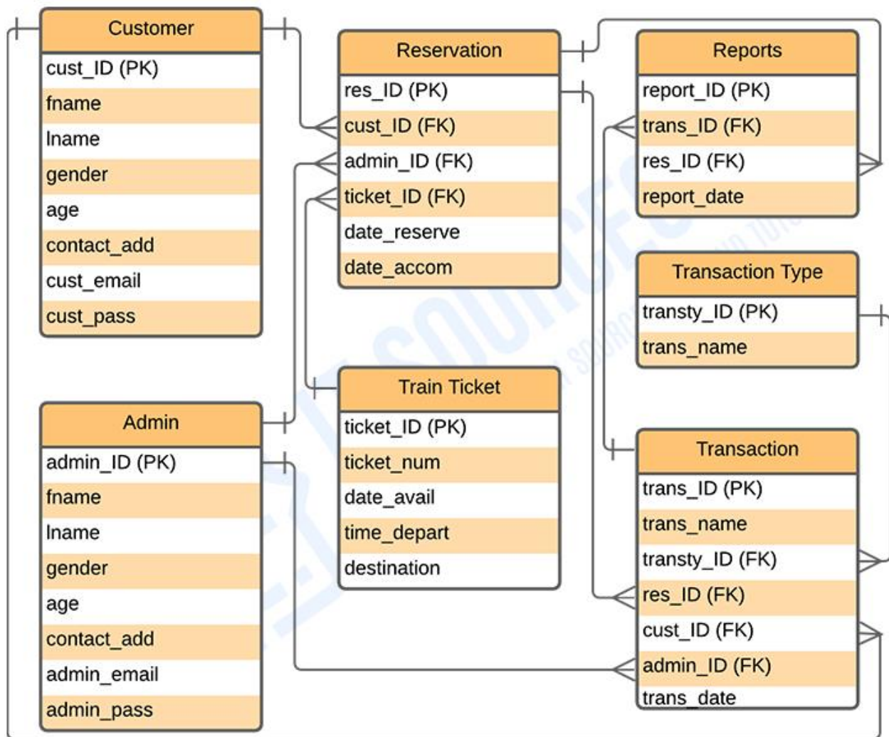
Railway Reservation System ER Diagram
