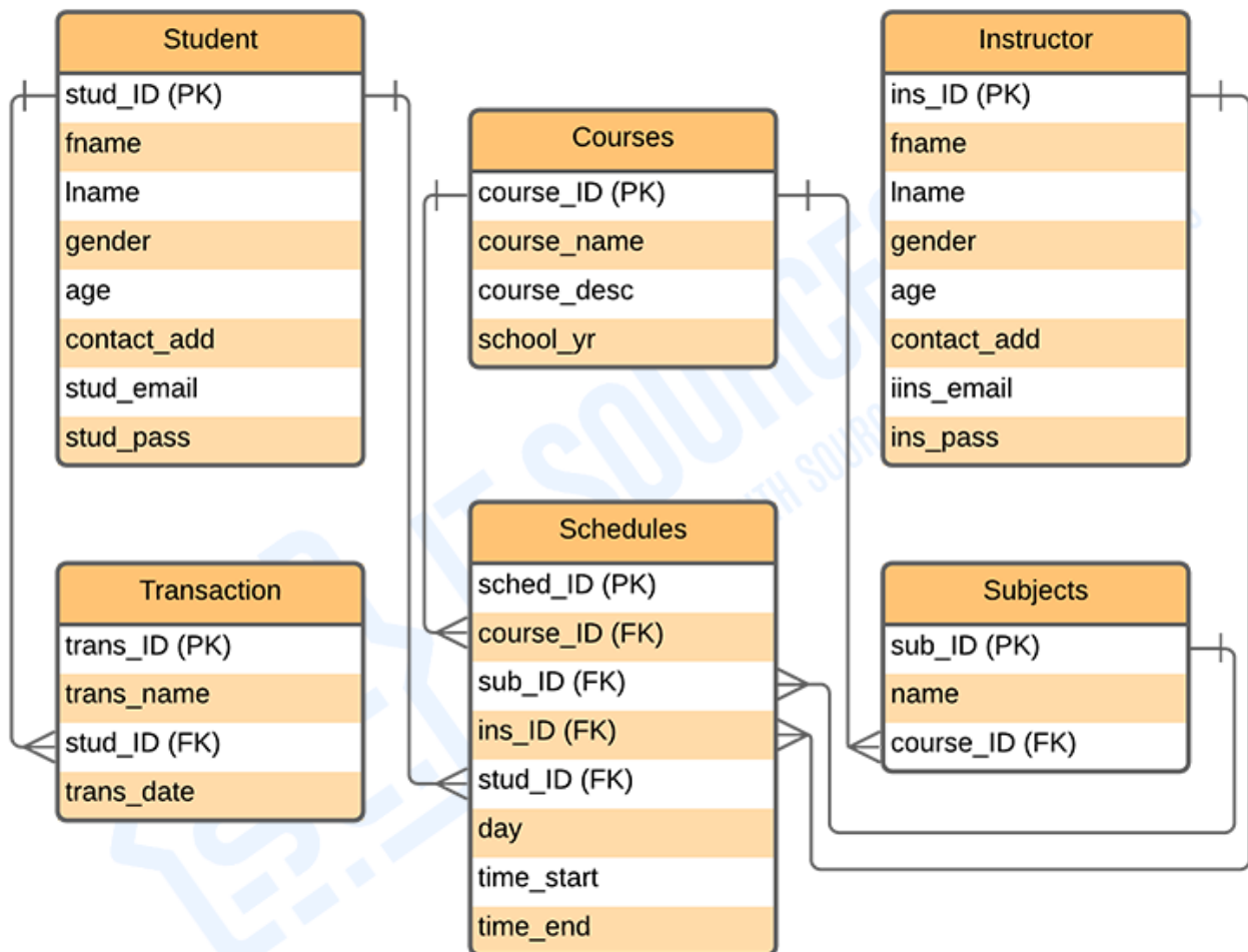
College Management System ER Diagram
