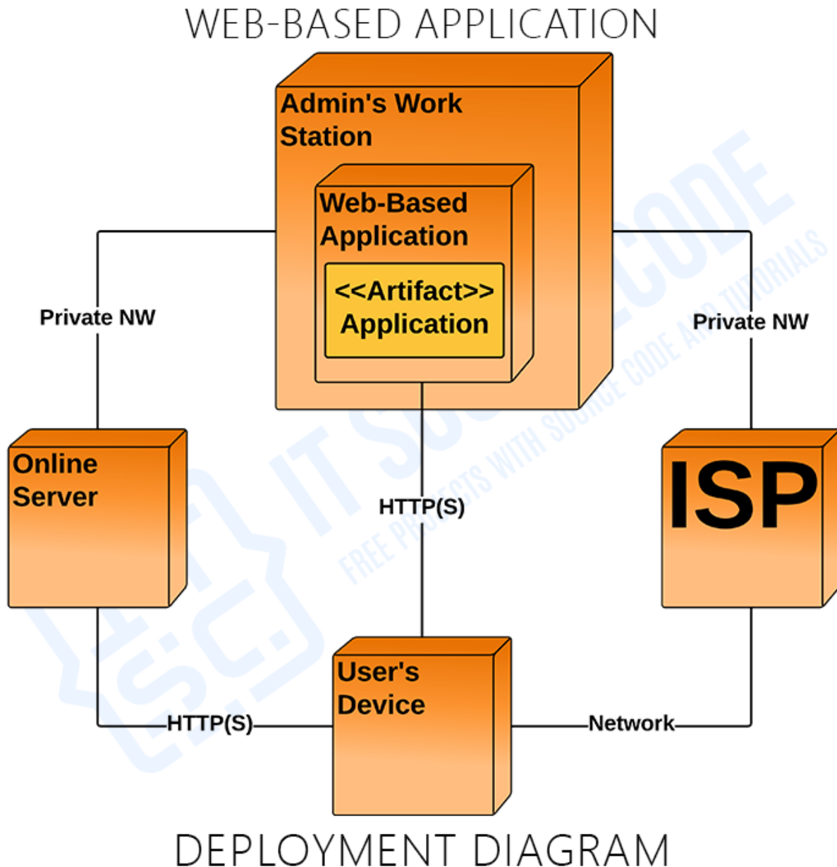
Deployment Diagram of Web Application in UML
